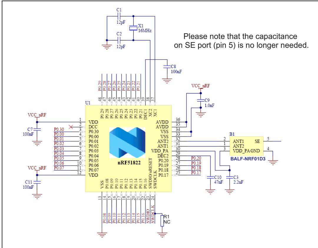
Figure 9. Application schematic
